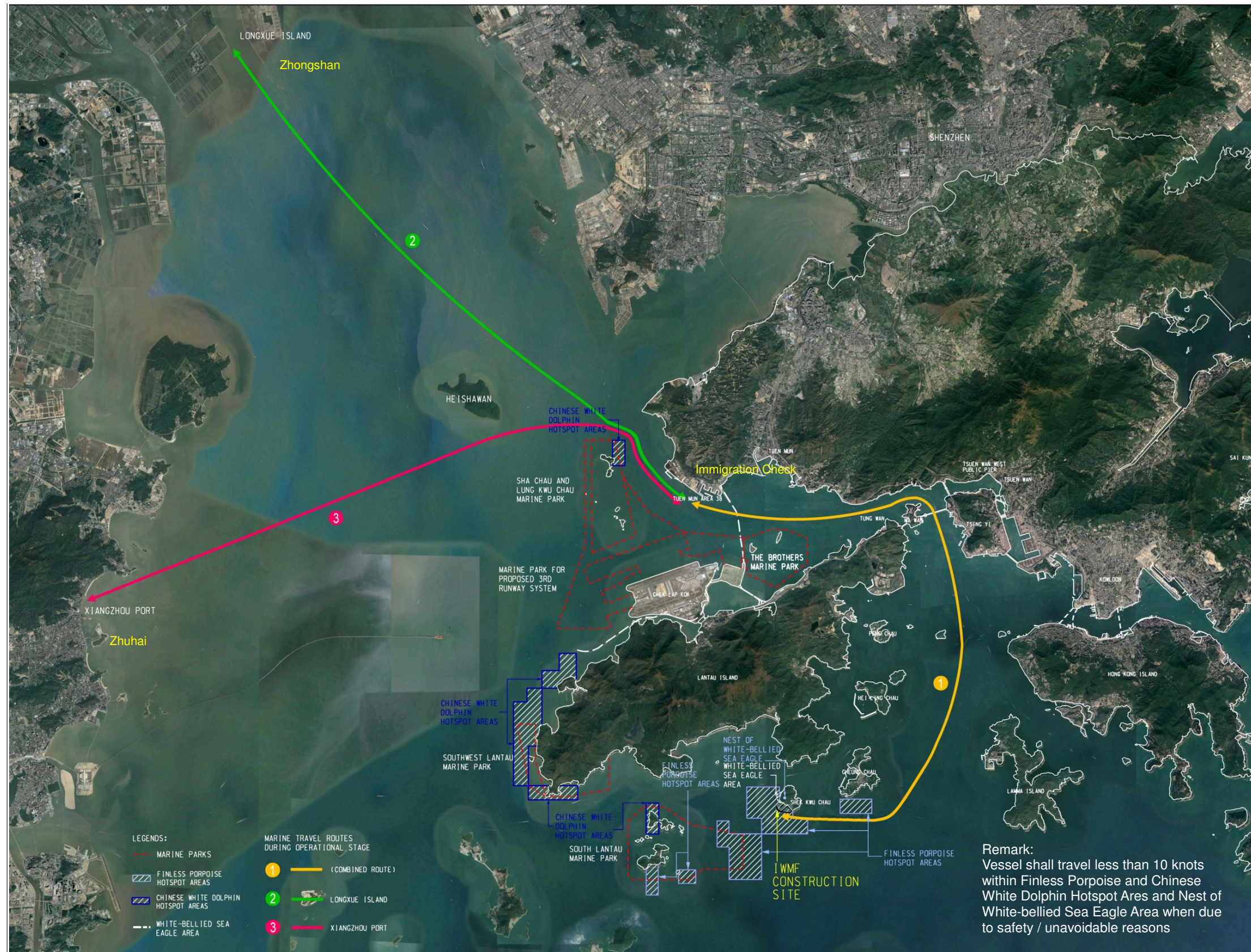
Figure 5 Marine Travel Routes for delivering Sand Fills from Zhongshan / Zhuhai, Guangdong to the construction site
